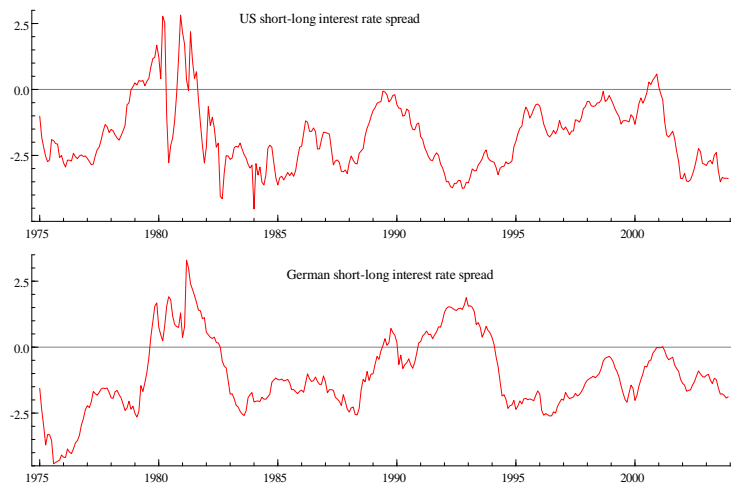
Figure 5: The graphs of the short-long interest spread for USA and Germany.
